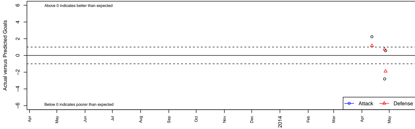
Fallbrook Villa FC B99 Dots are actual minus expected GF (blue circles) and GA (red triangles). Blue line is smoothed change in attack strength. Red is smoothed change in defense strength.
